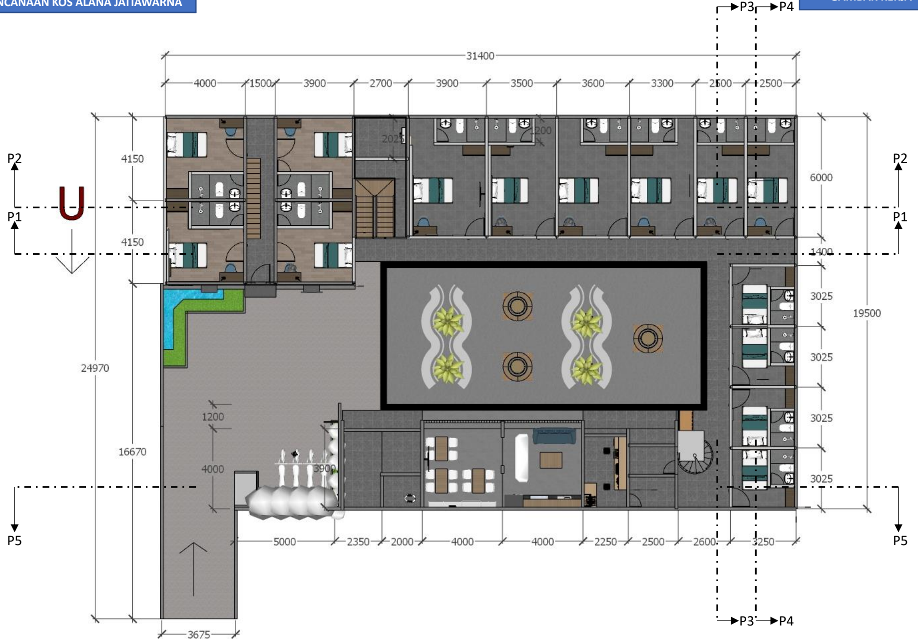
GAMBAR DENAH LANTAI 1
