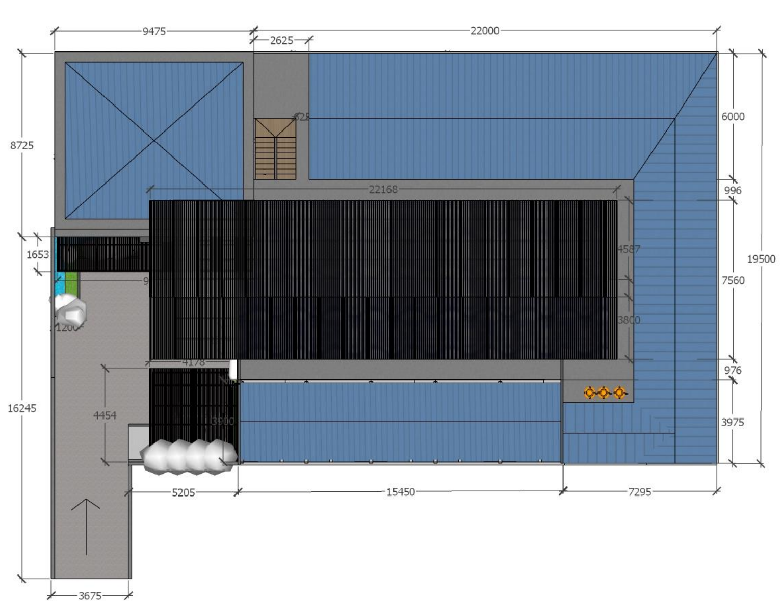
GAMBAR DENAH ATAP LANTAI 3
