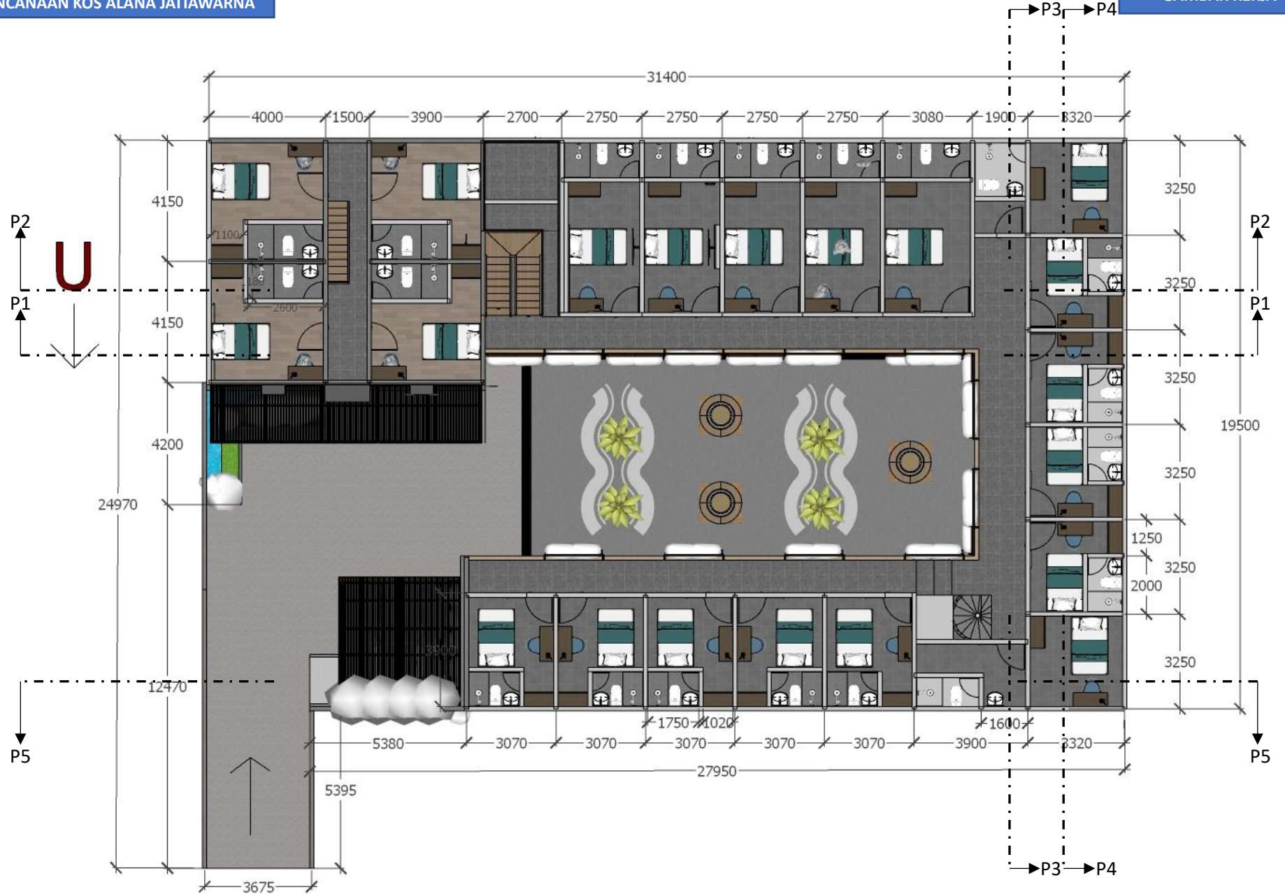
GAMBAR DENAH LAYOUT LANTAI 2
